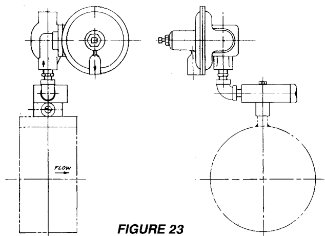
Pressure Reduction 1203 PILOT
