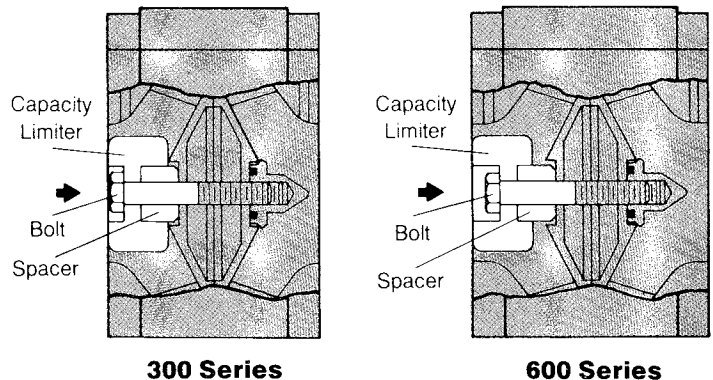
Installation drawing showing proper position of Capacity Limiter for 300 and 600 Series.
