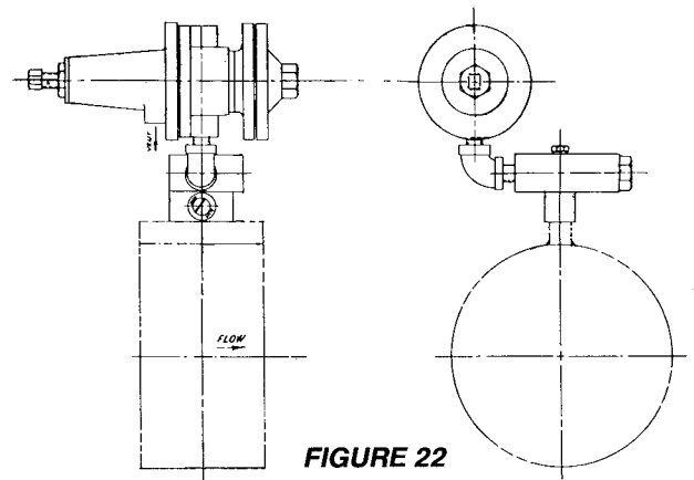
Pressure Reduction ZSC-100 and ZSC 320-100 PILOT
