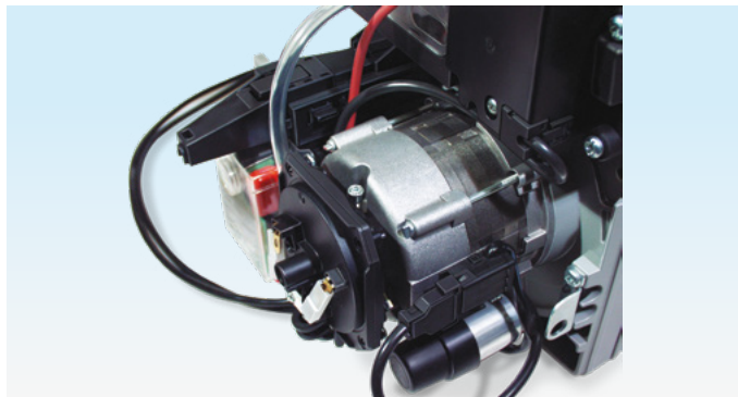
Pressure switch DL mounted on fan motor using a motor flange adapter
